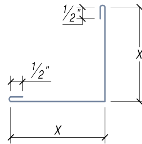
OUTSIDE CORNER
