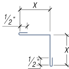
INSIDE CORNER
