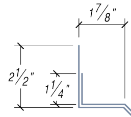
SILL
