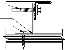
Floating Rakewall
