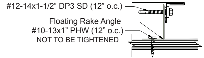
Floating Rakewall
