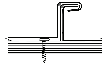
Cross Section 90° Seaming
