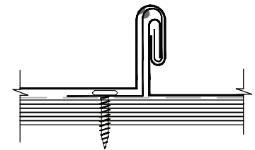
Cross Section 180° Seaming
