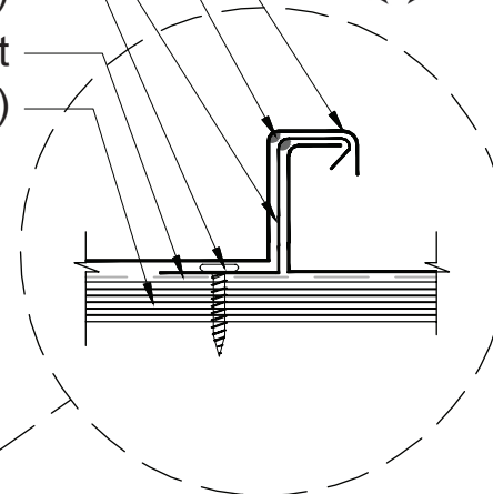
Cross Section Before Seaming
